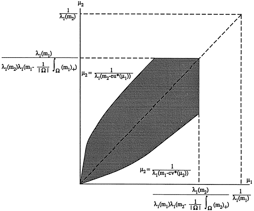
FIGURE 2.1. Permanence in (2.2) is guaranteed in the shaded region under the hypotheses of Theorem 2.1 when c < \int_{\Omega}(m_1)_+ / (|\Omega| \|(m_2)_+\|_{\infty}) and e < \int_{\Omega}(m_2)_+ / (|\Omega| \|(m_1)_+\|_{\infty}) .
