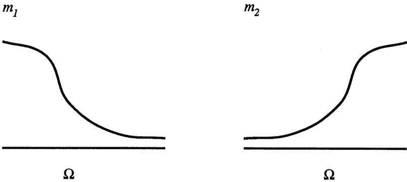
FIGURE 4.1. Profiles of growth rates for which permanence obtains in (4.1)–(4.2) for small diffusion rates under the assumption that b_{ij} \equiv 1 (strong competition).
